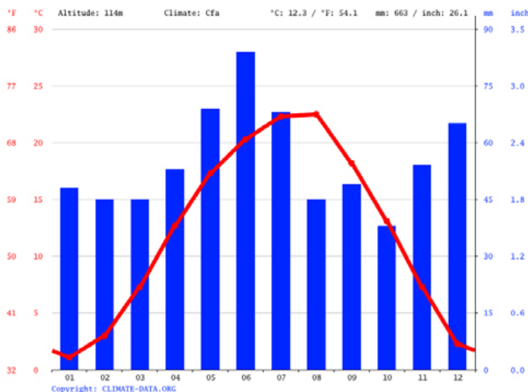
Figure 20: Climate graph
